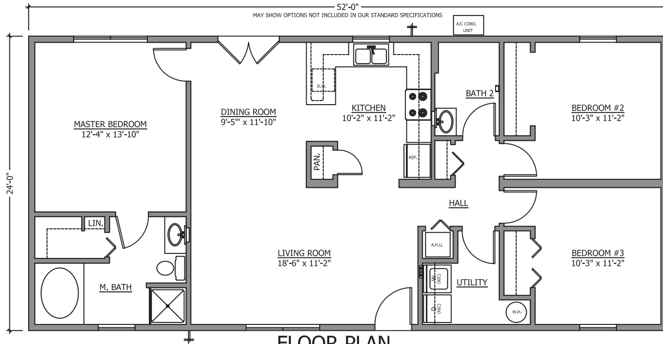
FLOOR PLAN
