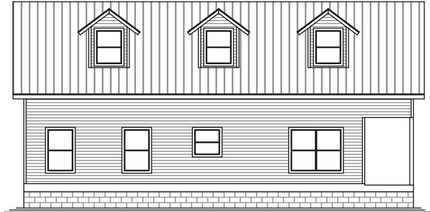
SIDE ELEVATION
